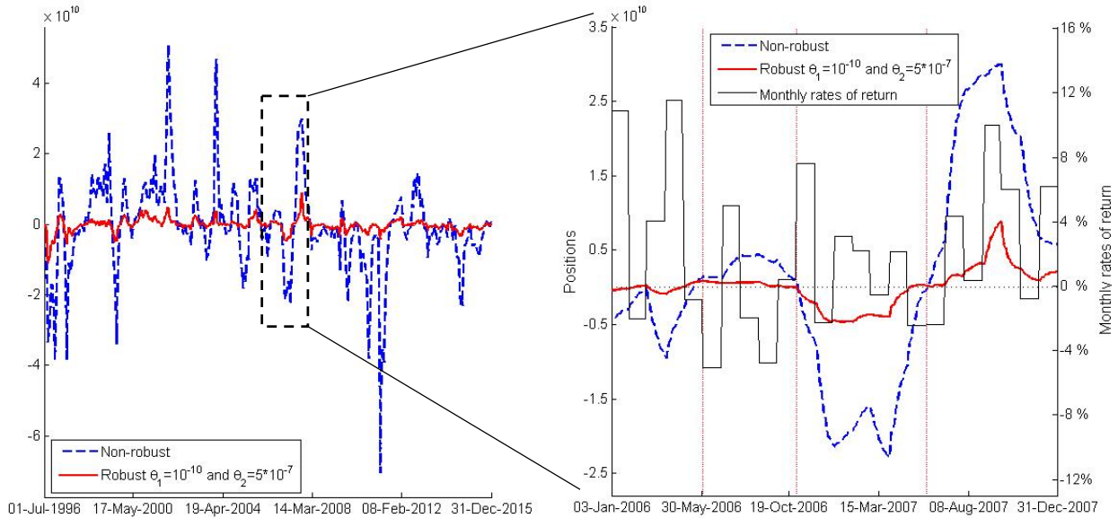
Figure 4-A: Gold positions of the robust and non-robust strategies
